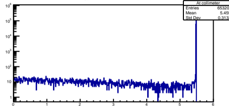
Lossed Energy in collimeter at Alpha (d = 9mm)
