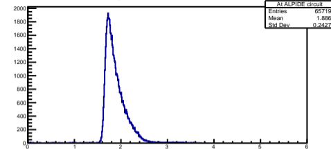
Lossed Energy in ALPIDE circuit at Alpha (d = 9mm)
