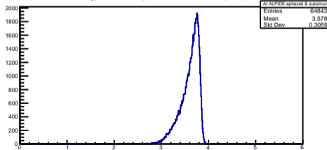
Lossed Energy in ALPIDE epitaxial + substruct at Alpha (d = 9mm)
