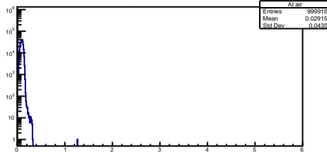
Lossed Energy in air at Alpha (d = 9mm)
